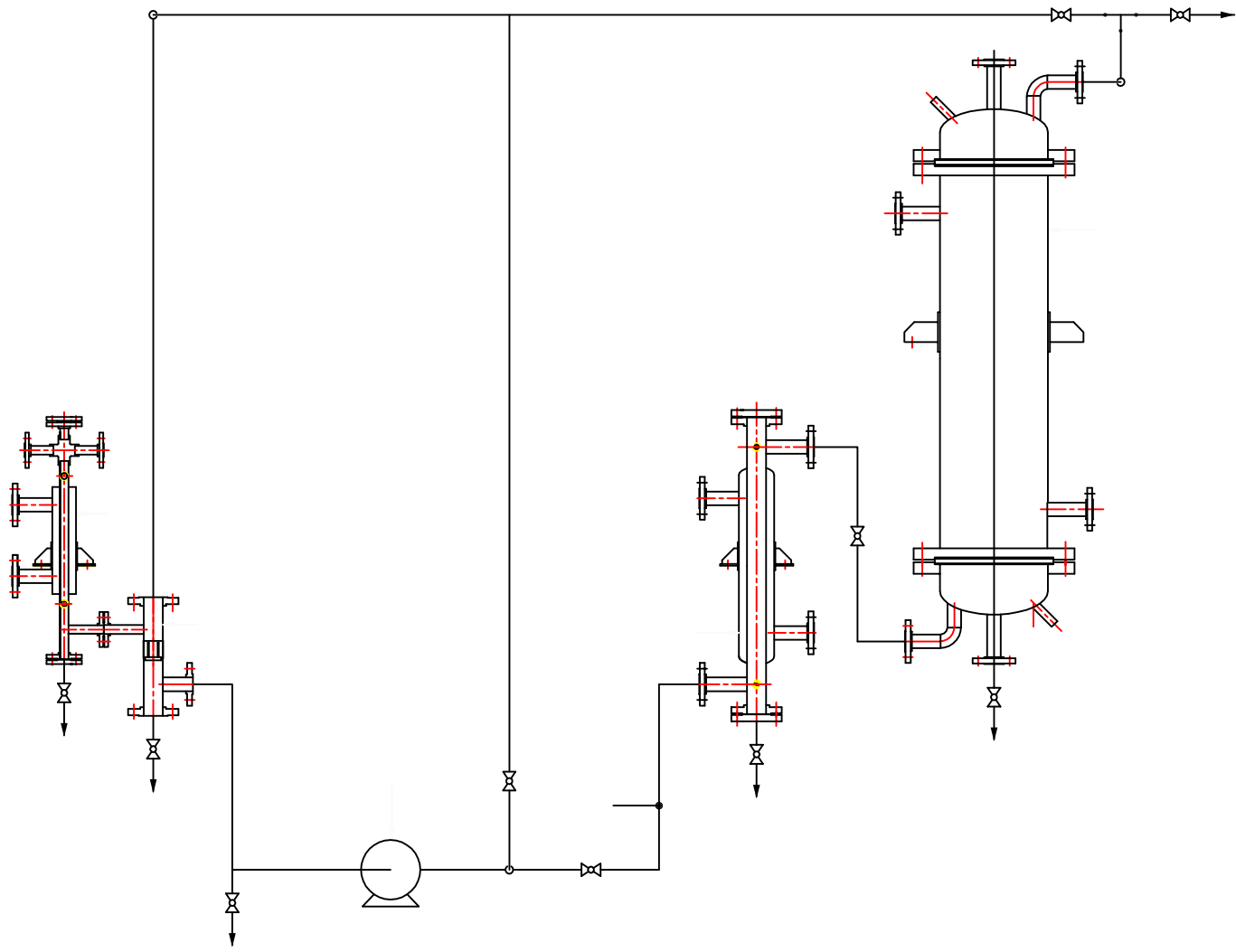
CONTINUOUS SULPHONATION REACTOR
