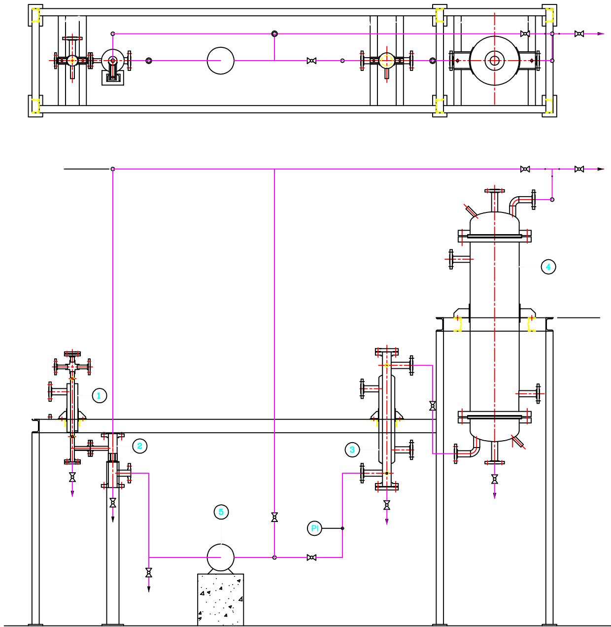
SULPHONATION REACTOR
